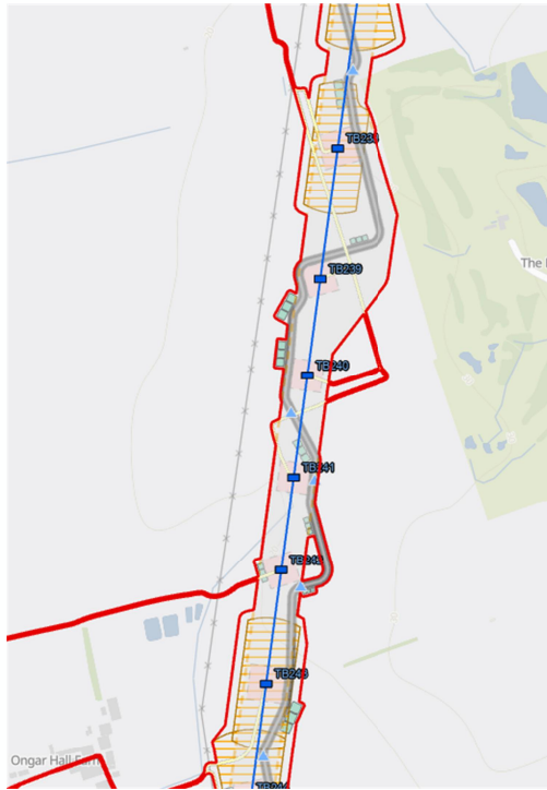
Figure 4.1: Proposed Project Design (document reference 6.4.F1) and Figure 4.2: Proposed Project Design – Permanent Features (document reference 6.4.F2) show an alignment between TB238 and TB243. Low height pylons are proposed between TB238 and TB243 to cater for Thurrock Airfield. However, should a housing development be brought forwards at Thurrock Airfield and/or the airfield be closed, low height pylons would not be required and standard lattice pylons would be installed instead.
